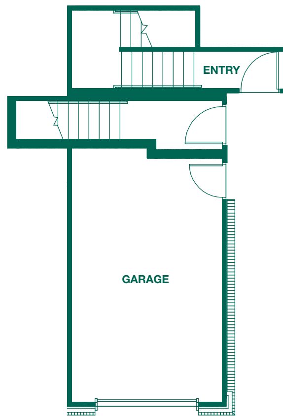
GARAGE FLOOR PLAN
